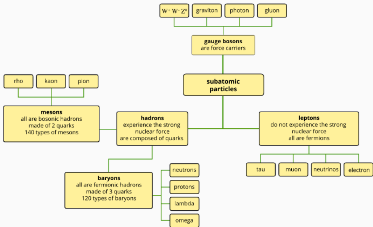
9.1.3 • This mind map summarises the classification of particles in the Standard Model of particle physics.
