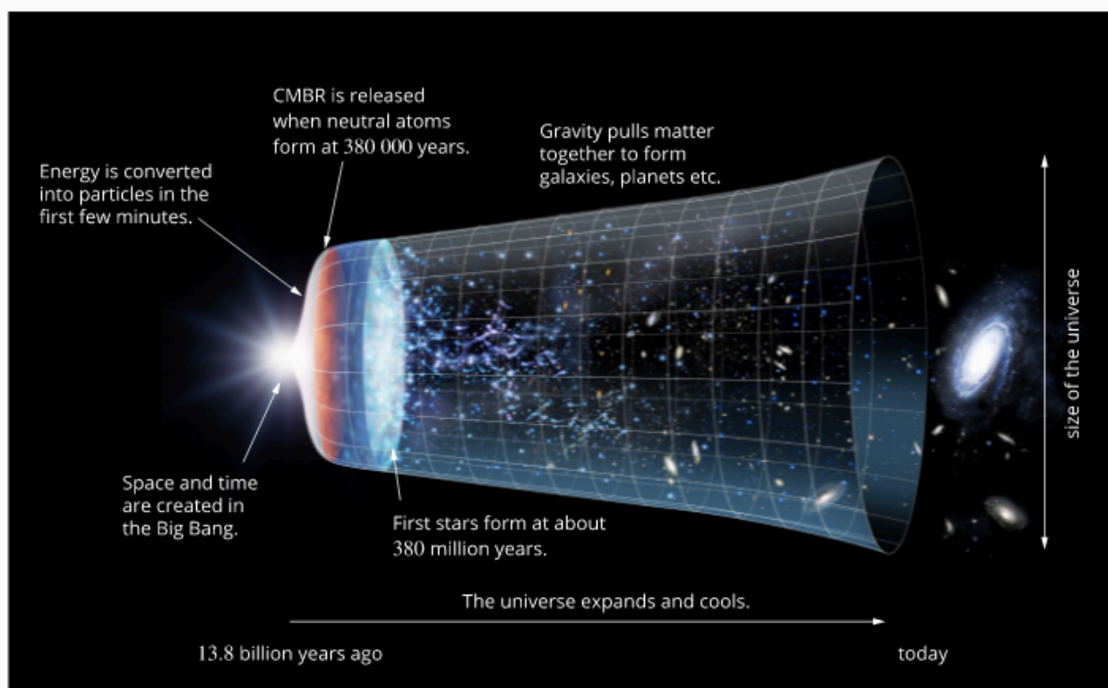
9.4.14 • The 13.8 billion year history of the universe. (Not to scale!)
