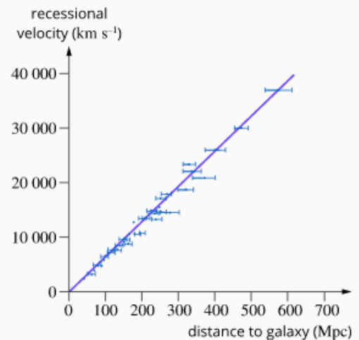
9.4.6 • Hubble discovered that the galaxies were receding from us at velocities proportional to their distance. The slope of the line is known as Hubble's constant, H_0 .
